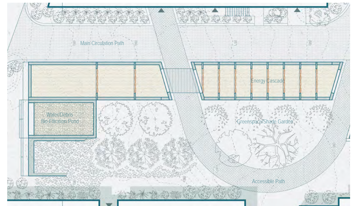
Figure 43. Stores lower greenspace detail - Plan. 2022, by author. (not to scale on a 8.5x11 sheet)
